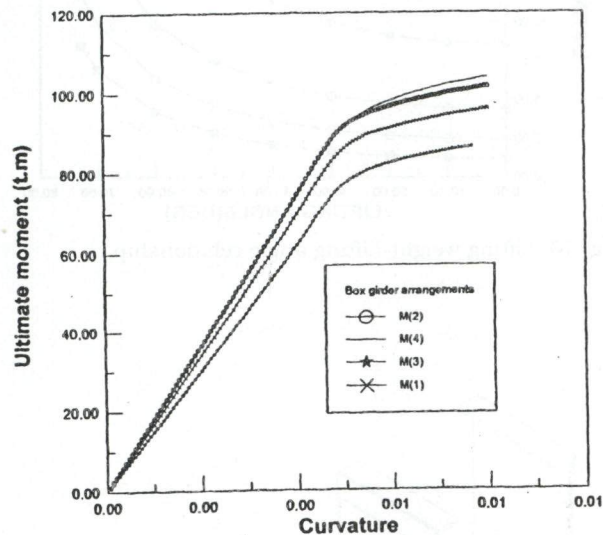
Fig. 8. Ultimate moment-curvature relationship of the crane boom.
