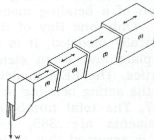
Fig. 5. Typical profile of the telescopic crane boom.
