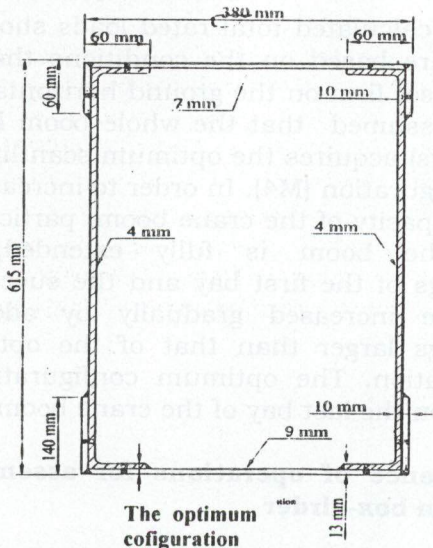
Fig. 9. Optimum configuration of the boom cross section.
