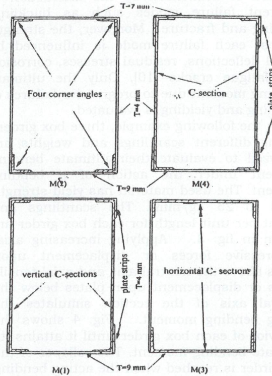
Fig. 6. Proposed configurations of the boom box girder.
