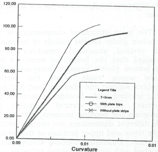
Fig.4 Ultimate moment-curvature relationship of the box girder.
