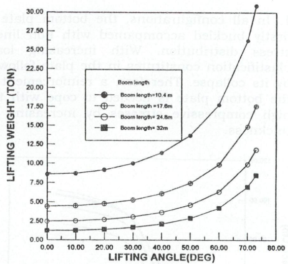
Fig. 10. Lifting weight-Lifting angle relationship.
