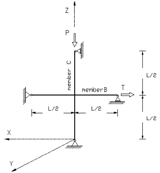
Hinged and roller supports at members B and C ends
