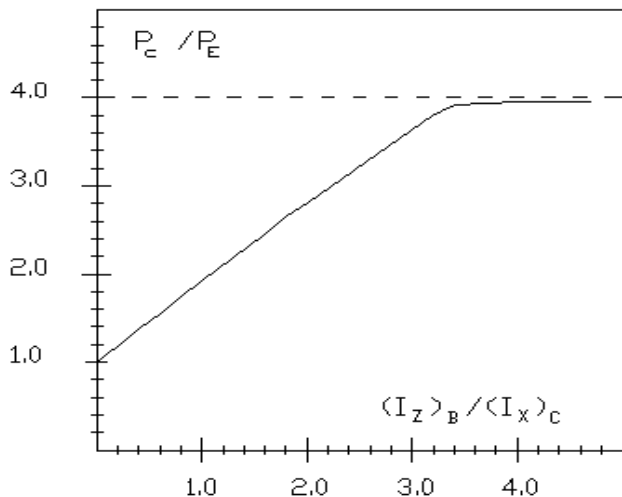
Fig. 2. Relation between P_C/P_E and (I_Z)_B/(I_X)_C when (I_Y)_C/(I_X)_C = (I_Y)_B/(I_X)_C = 1 .
