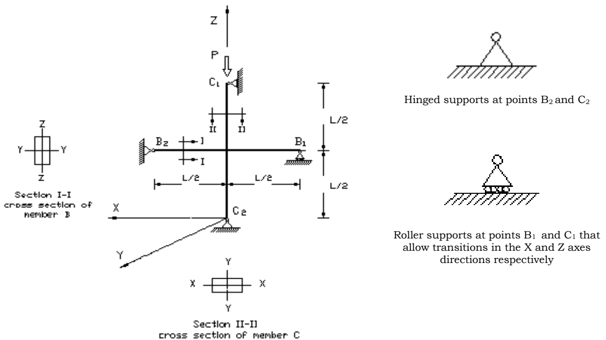
Fig. 1. Finite element model of cross bracing members.
