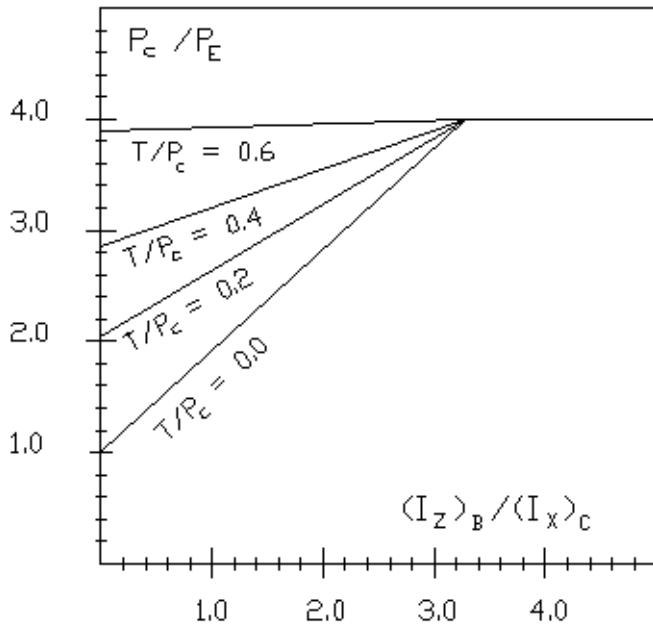
Fig. 8. Relation of P_c/P_E and (I_z)_B/(I_x)_C at different values of T/P_c .
