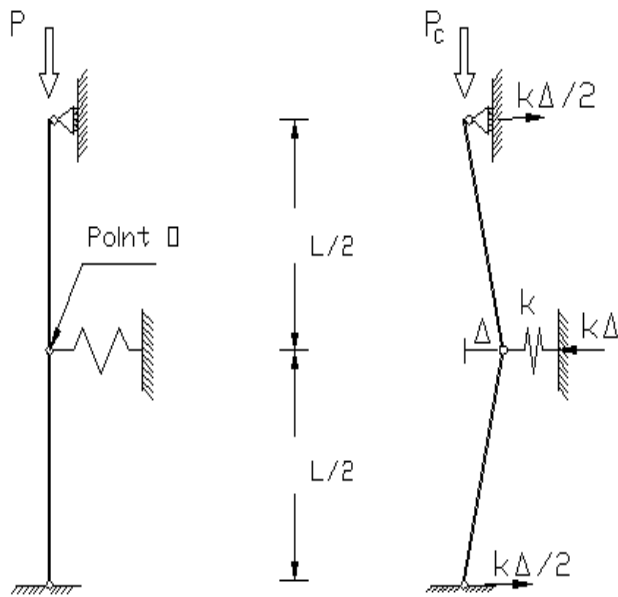
Fig. 6. Model of hinged - hinged column supported by spring at its mid length.
