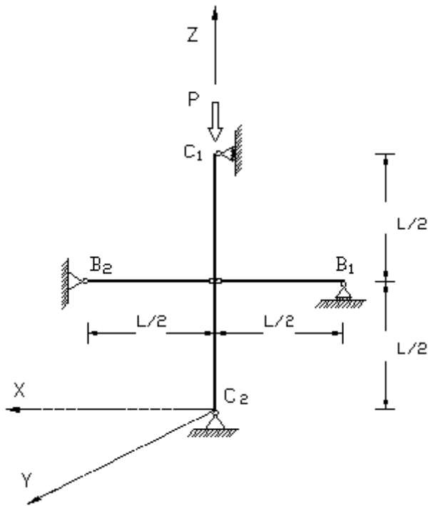
Fig. 5. Finite element model when member B is hinged to member C.
