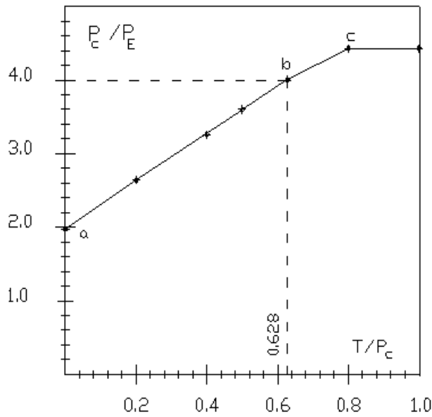
Fig. 4. Effect of tension load T in member B on the out of plane buckling load P c .
