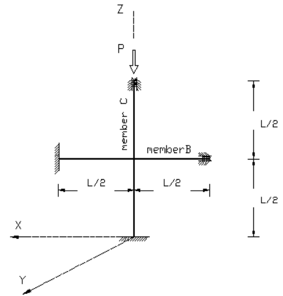
Fixed-fixed supports at members B and C ends
