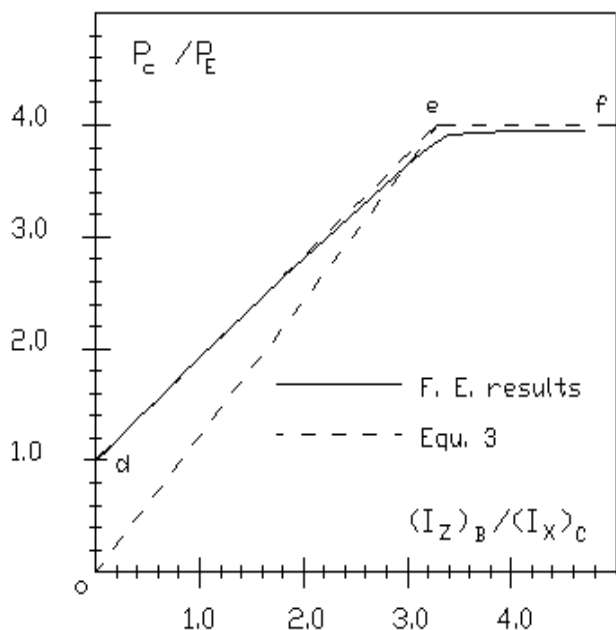
Fig. 7. Comparison between finite element and analytical models results.
