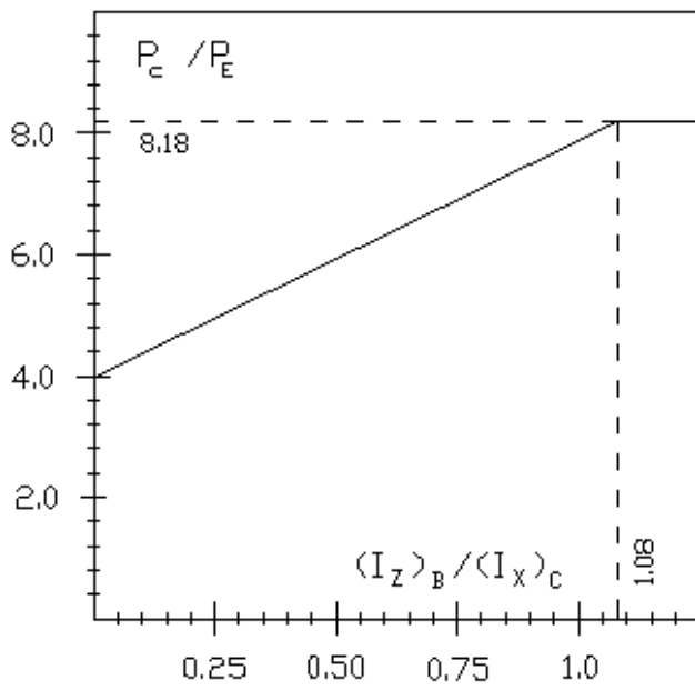
Fig. 9. Relation of P_c/P_E and (I_z)_B/(I_x)_C when fixed supports at members B and C ends.
