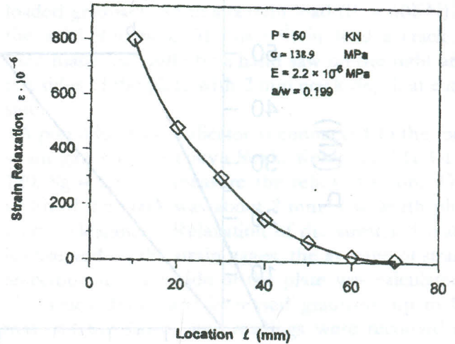
Figure 8. Relationship between relaxed strain & crack location.
