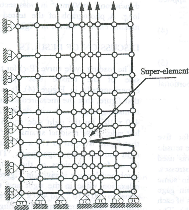
Figure 2a. Mesh for one quarter specimen.
