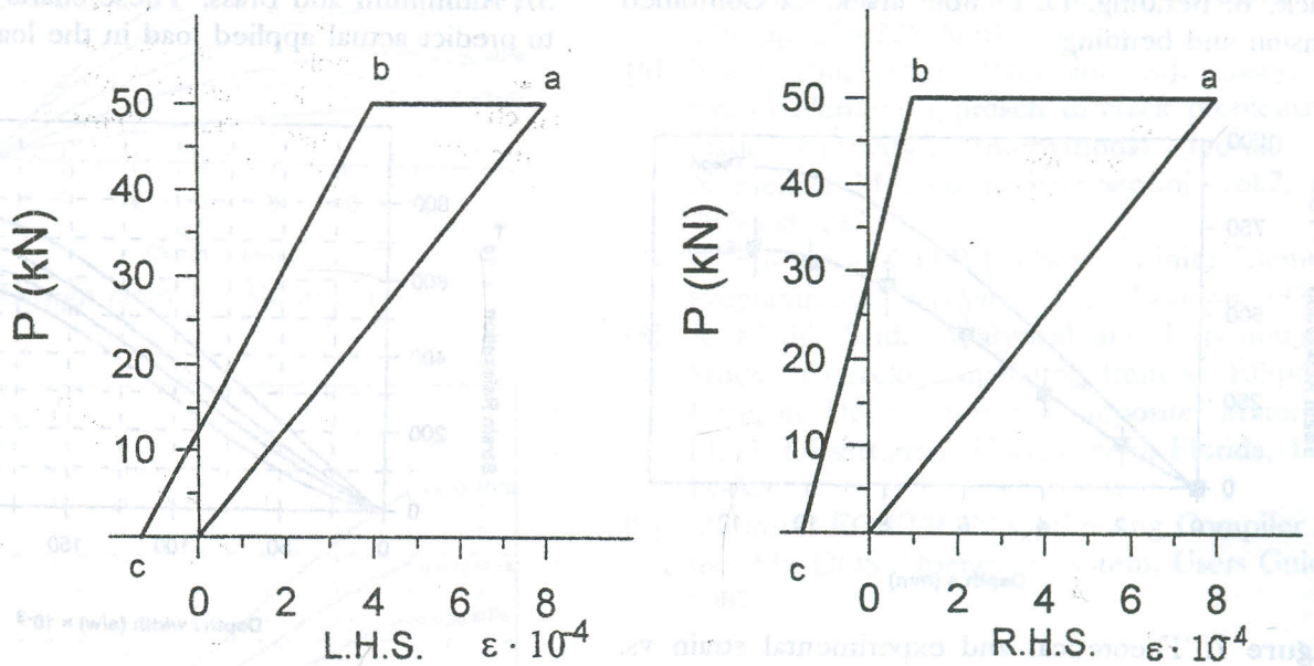
Figure 5. Strain relaxation vs. combined load for two single edge cracks.
