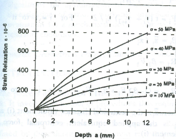
Figure 10. Design chart for Aluminum.
