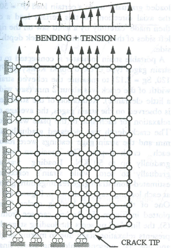
Figure 1a. Mesh for one quarter specimen.
