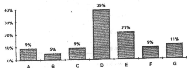
Figure 10. Longitudinal distribution of fractures along the bottom structure.
