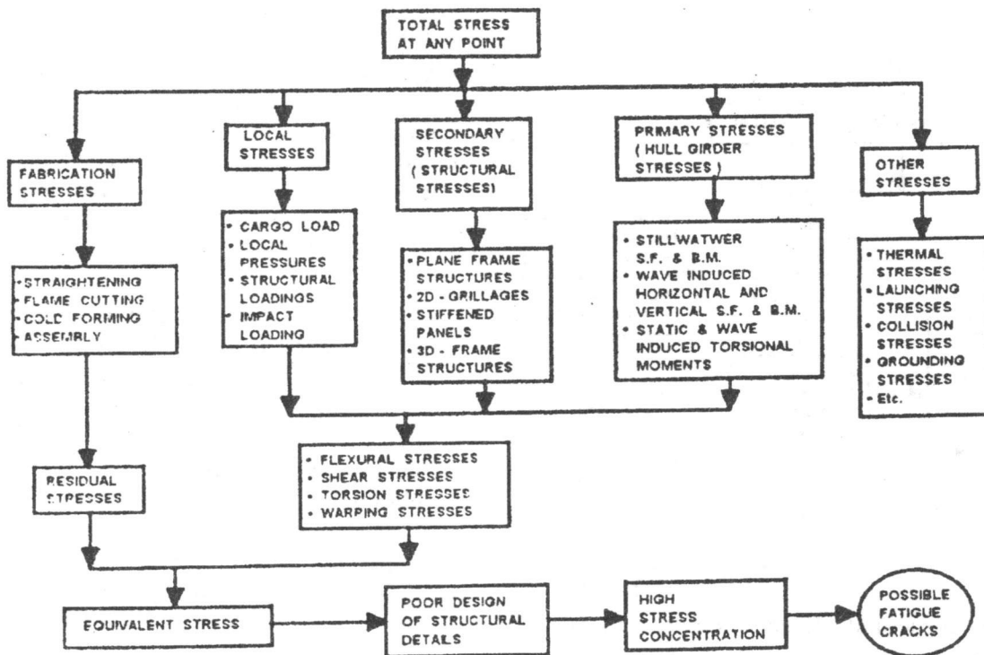
Figure 23. Total stress at any point.
