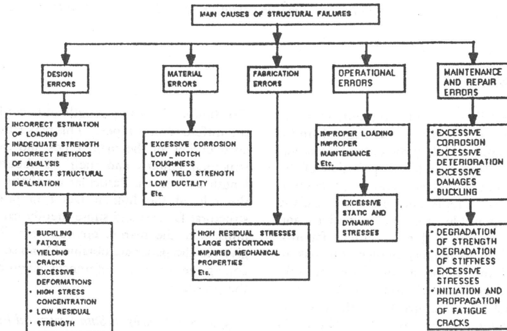
Figure 1. Main causes of structural failures.
