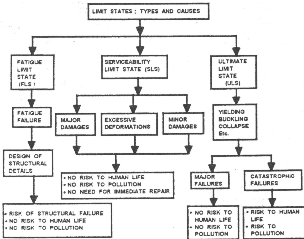
Figure 3. Limit states; types and causes.
