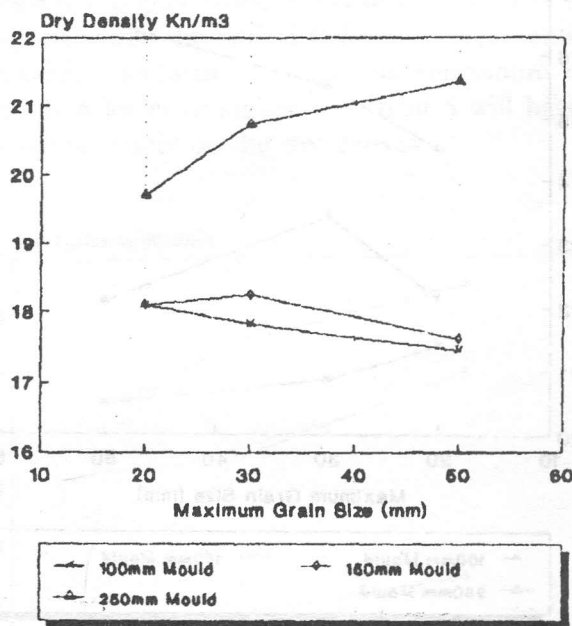
Figure 3. Compaction test for Crushed lime stone aggregate
