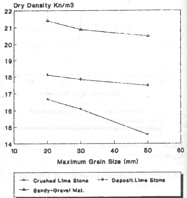
Figure 5. Compaction test using mould diameter 100mm.
