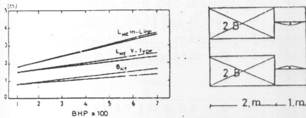
Figure 6. Dimensions of main engine.
