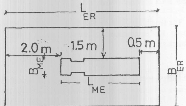
Figure 7. Engine rooms dimensions.
