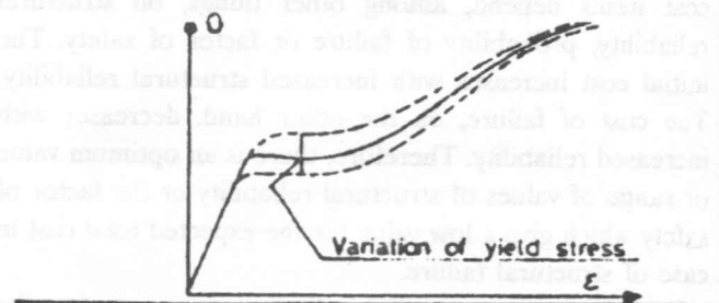
Figure 2. Stress-strain diagram.
