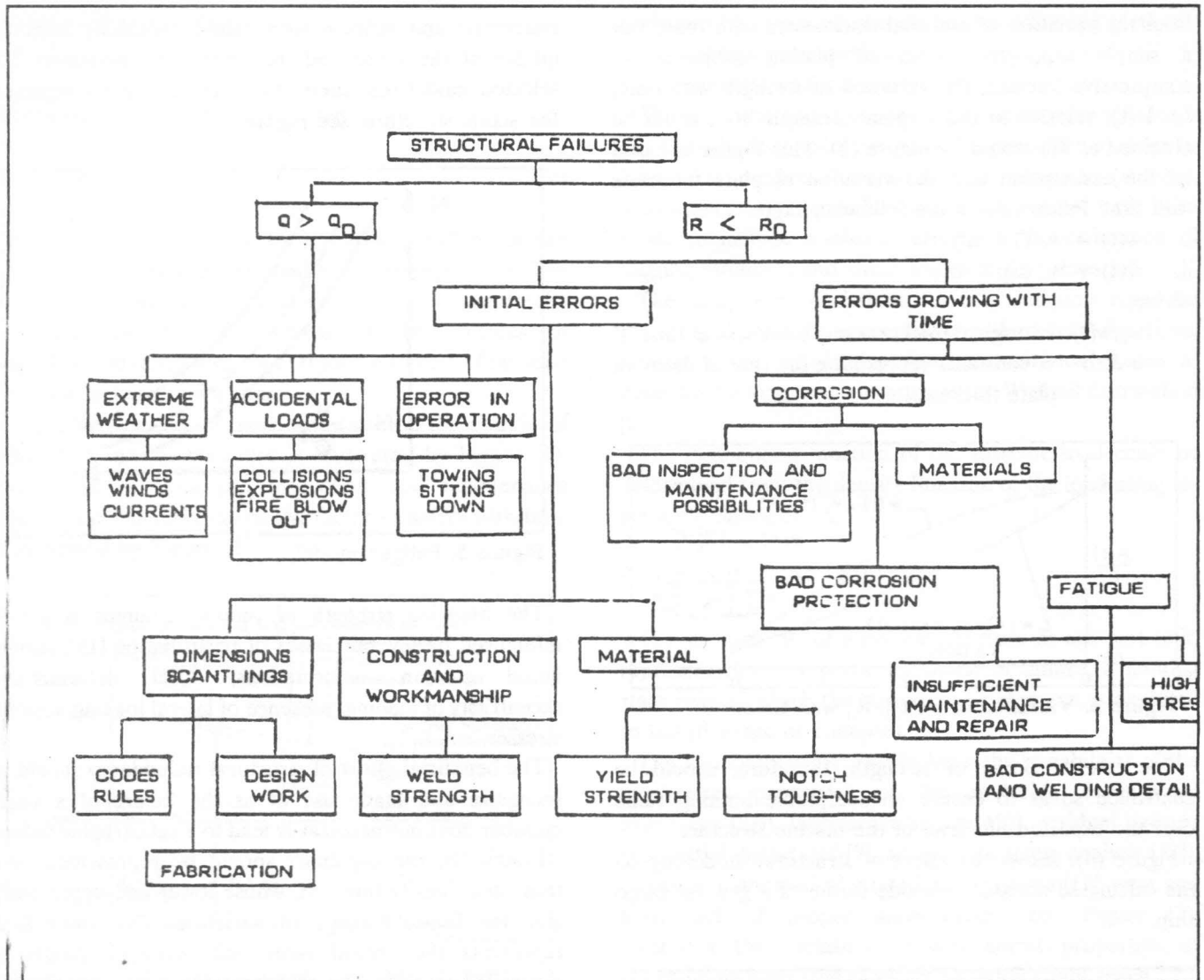
Figure 6. Various causes of structural failure.
