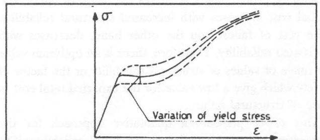
Figure 2. Stress-strain diagram.
