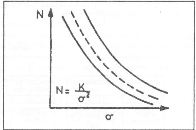
Figure 5. Fatigue model.
