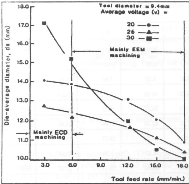
Figure 4. Variation in die-average diameter with tool feed rate for three average voltages.
