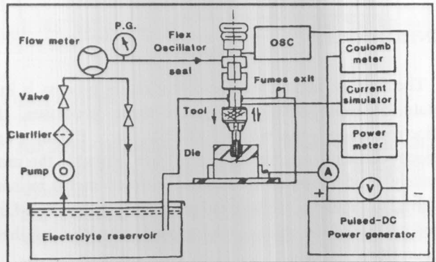
Figure 3. A schematic of EEDM die-sinking.
