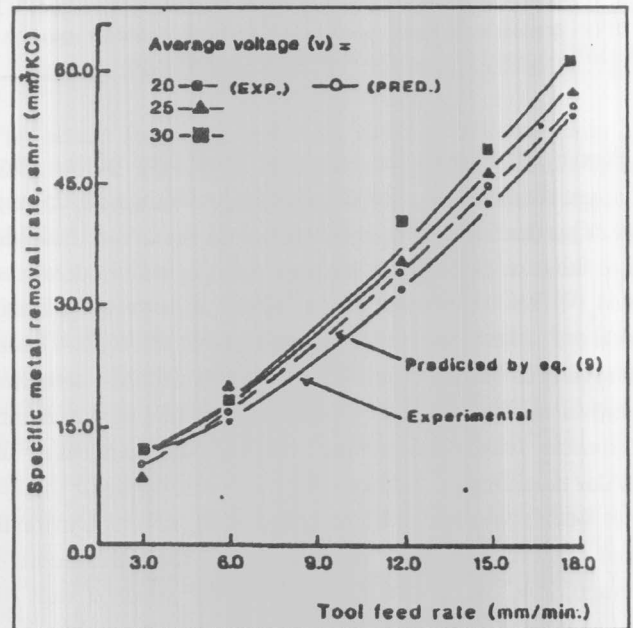
Figure 6. Variation in smrr with tool feed rate for three average voltages.
