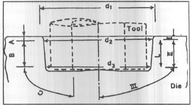
Figure 2. Die measured sections and distribution of machining regions.
