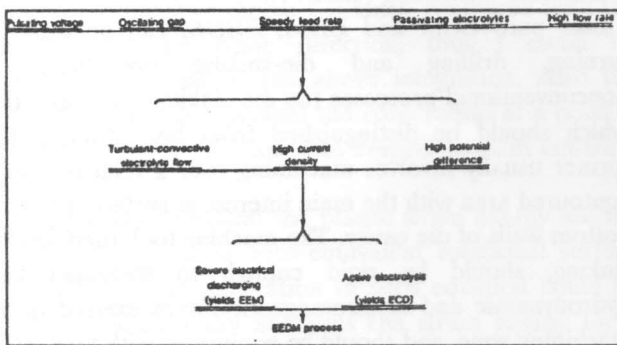
Figure 1. Combination of variables which yield machining by EEDM.
