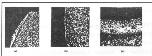
Figure 9. Optical microscopy sections at die entrance (a), midheight (b) and central bottom (c).
