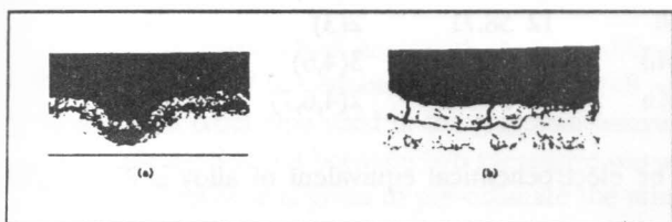
Figure 10. Pitted surface by ECD at die side walls (a) and white damaged layers with micro and microcracks (b).
