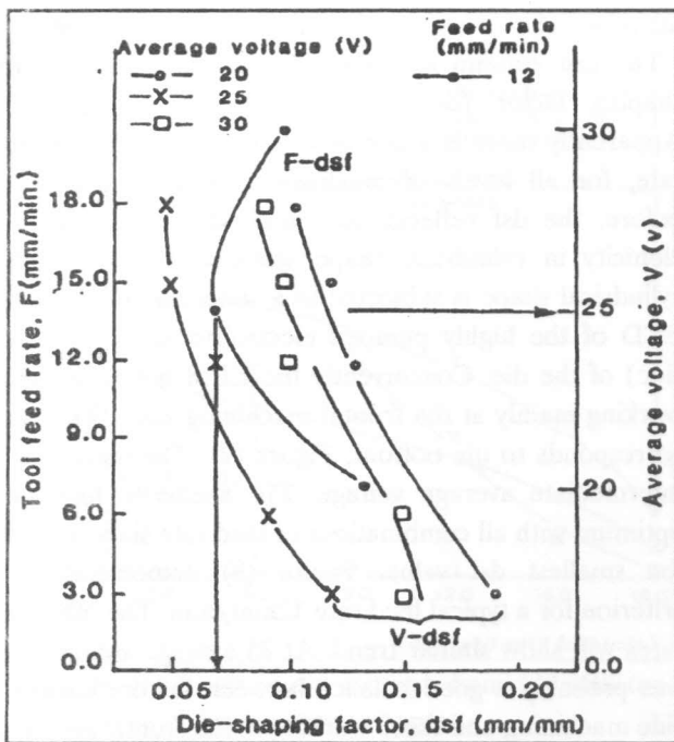
Figure 8. Variation in die-shaping factor with average voltage and one typical optimum feed rate 12mm/min.
