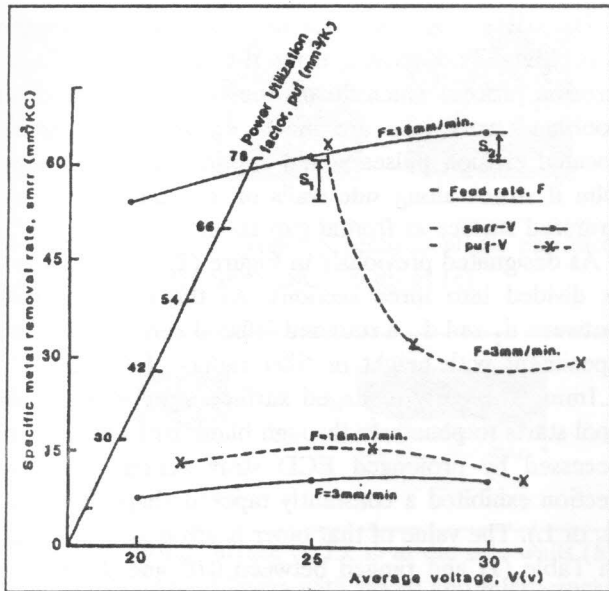
Figure 7. A 3-D experimental relationship of smrr and puf, as a function of voltage with the highest and lowest feed rates 3 and 18mm/min.
