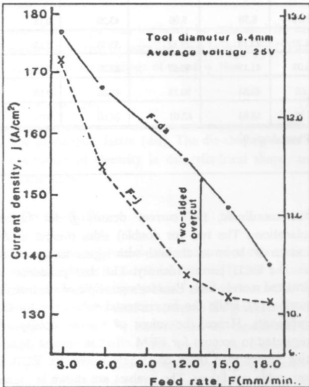
Figure 5. Effect of feed rate on current density and die-average diameter with average voltage 25V.
